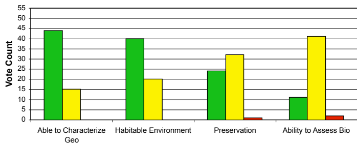
Eberswalde Crater
