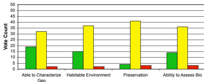
Ritchey Crater
