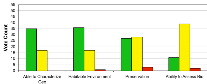
Holden Crater
